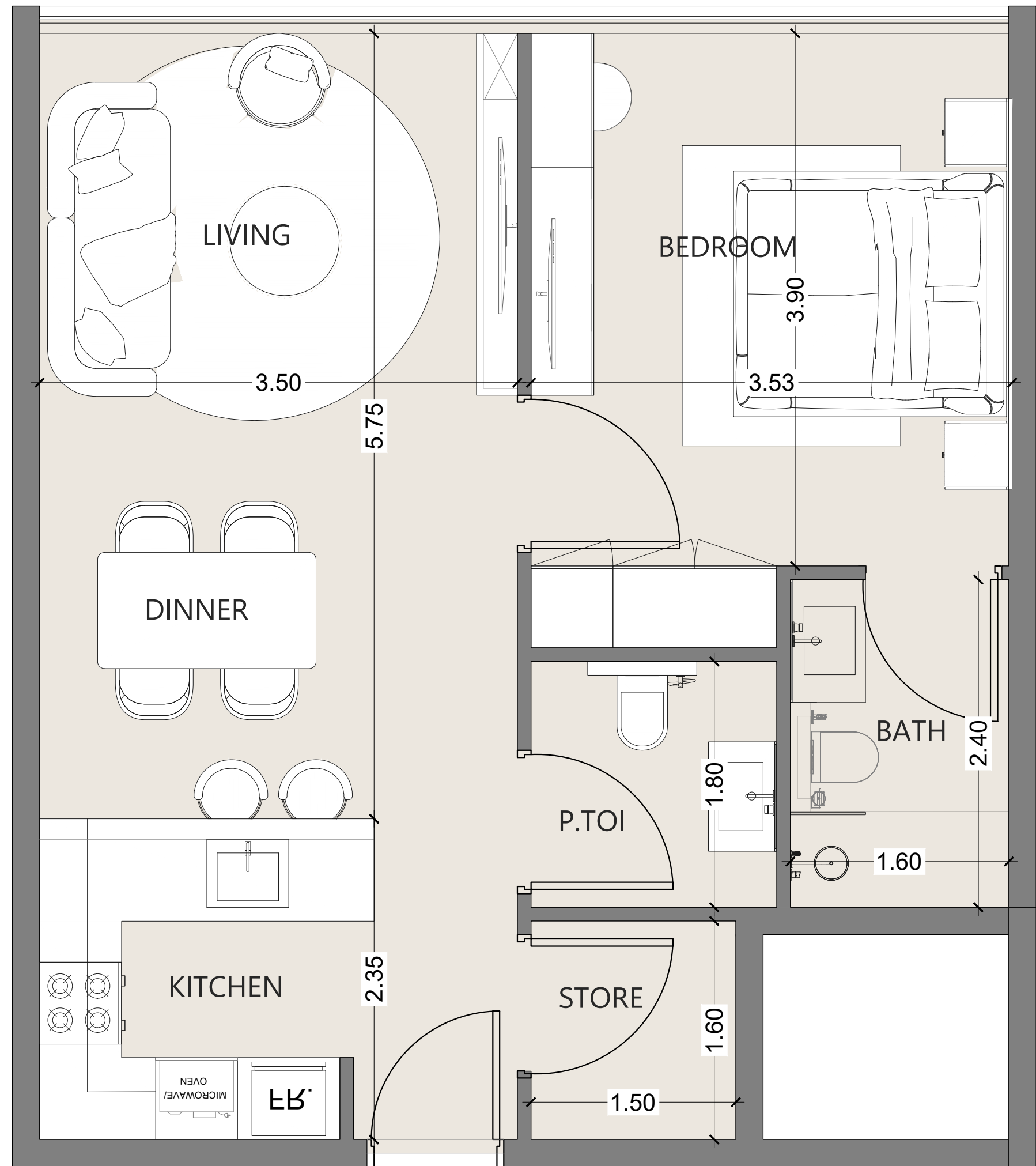
1BHK B,C&D NET AREA 733.45 SQ.FT AVG. BALCONY AREA 117.86 SQ.FT
